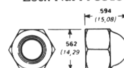
Acorn Lock Nut M-3236
