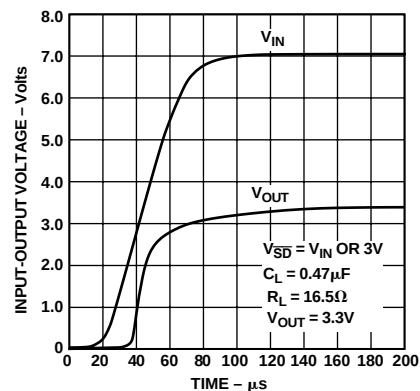
Figure 10. Power-Up Transient
