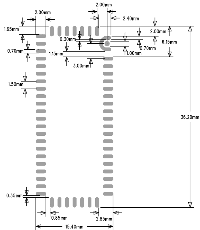
Figure 6: Dimensions of WT41
