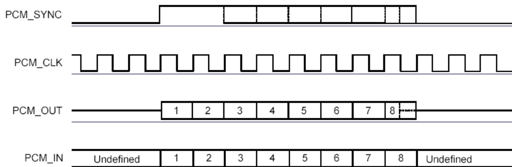
Figure 21: Long Frame Sync (Shown with 8-bit Companded Sample)
