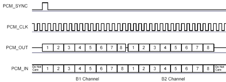
Figure 24: GCI Interface
