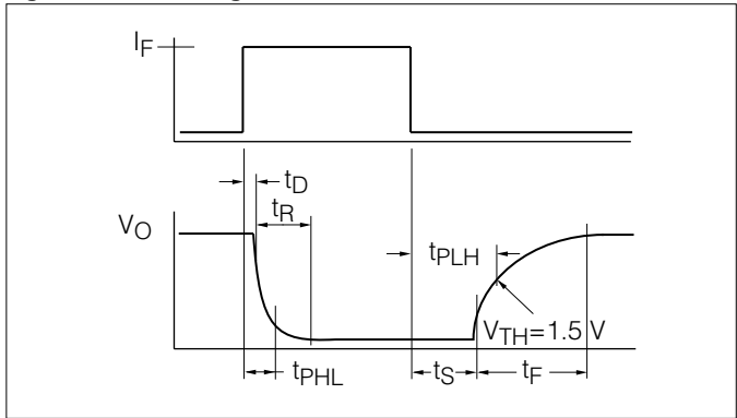
Figure 9. Switching waveform
