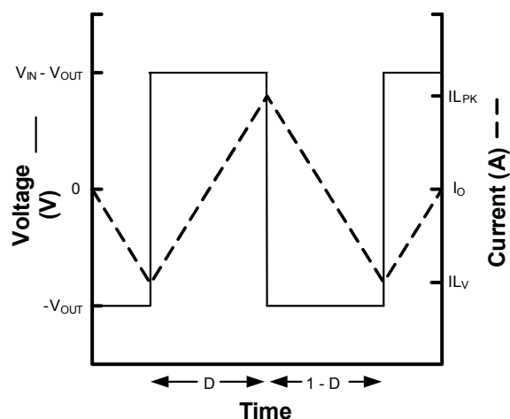
FIGURE 11. INDUCTOR WAVEFORM
