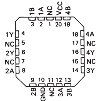
SN54LS386A . . . FK PACKAGE (TOP VIEW)
