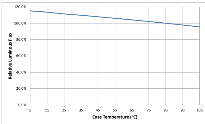
Relative Output Flux vs. Case Temperature
