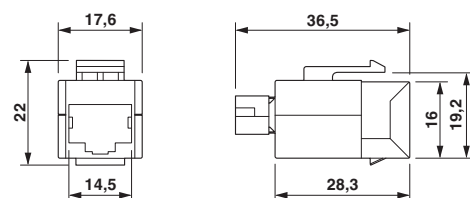
RJ45 socket insert, keystone
