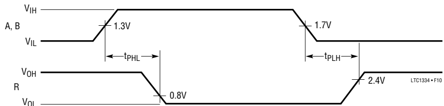
Figure 10. RS232 Receiver Propagation Delays
