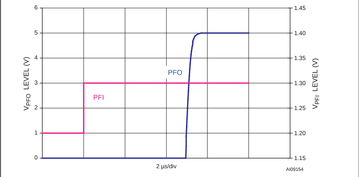
Figure 25. Power-fail Comparator Response Time (De-Assertion)
