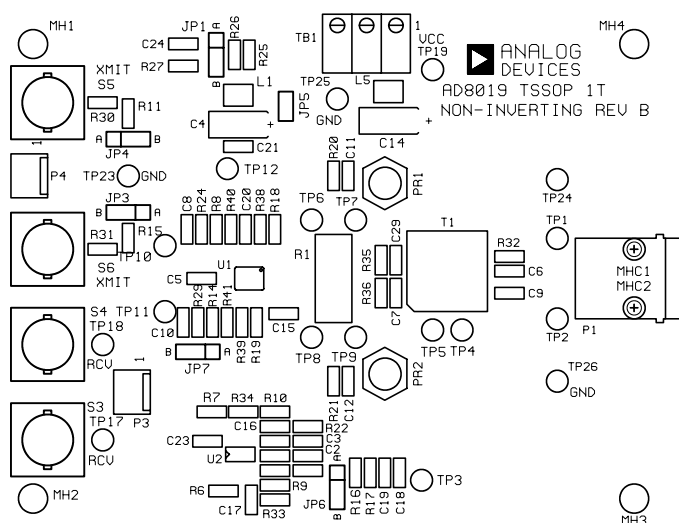
Figure 10. TSSOP Evaluation Board Silkscreen Top
