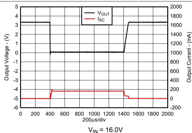
Figure 5-17. Short-Circuit Current vs Time (New Chip)
