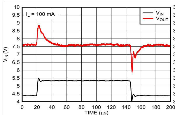
Figure 5-13. Line Transient Response (New Chip)
