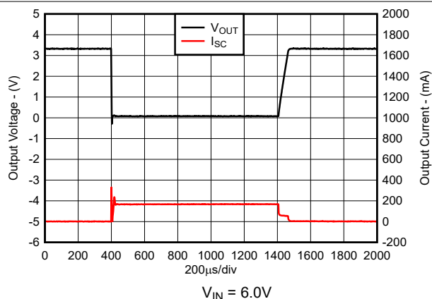
Figure 5-16. Short-Circuit Current vs Time (New Chip)
