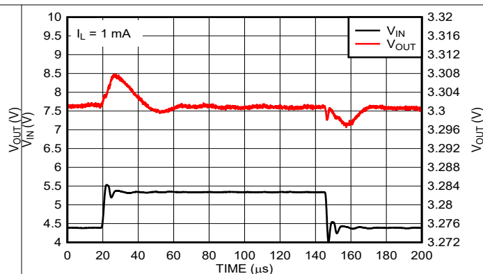
Figure 5-14. Line Transient Response (New Chip)
