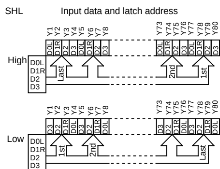
Figure 4 Column Driver Operating Mode
