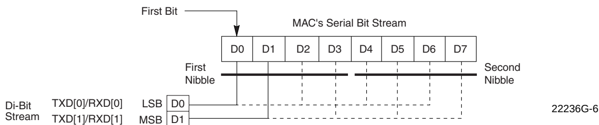
Figure 4. Bit Ordering
