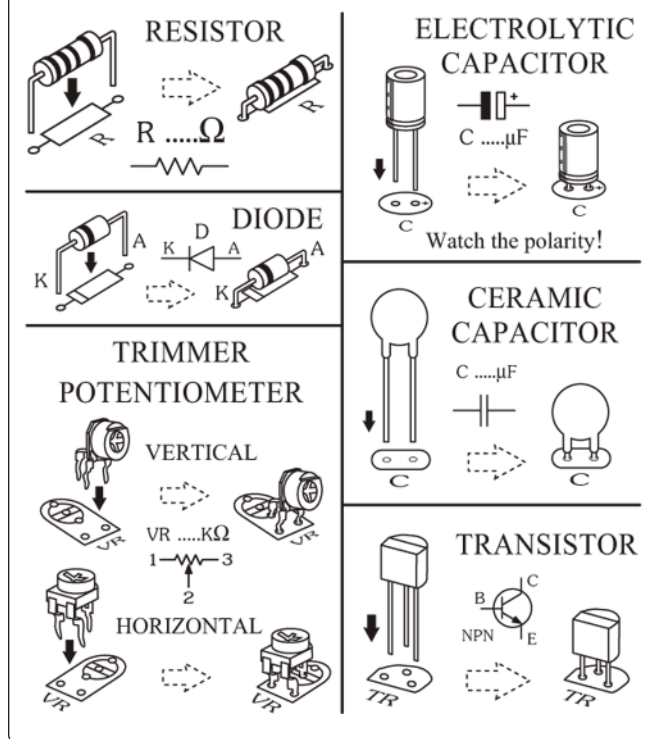
Figure 1 Installing components
