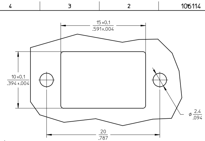
RECOMENDED MOUNTING PATTERN
