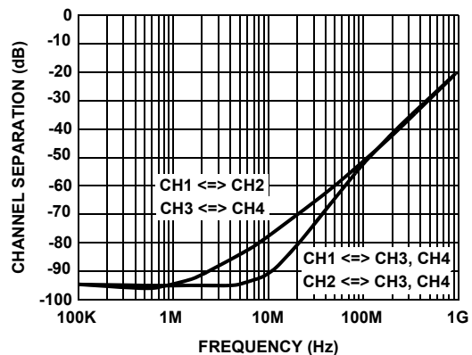
FIGURE 20. CHANNEL SEPARATION vs FREQUENCY (EL8401)
