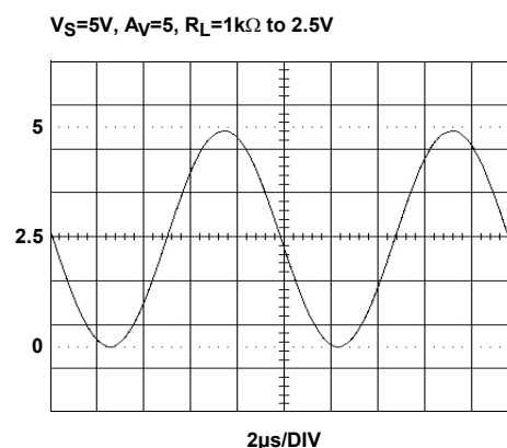
FIGURE 24. OUTPUT SWING
