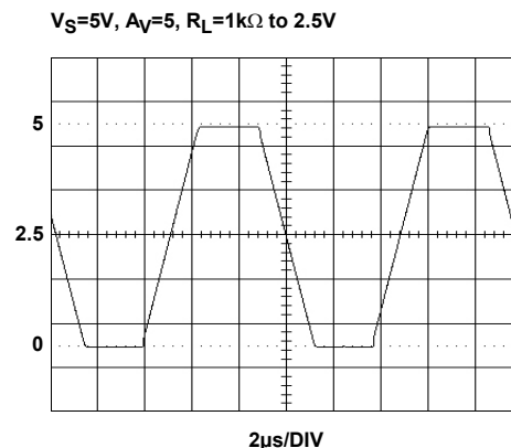
FIGURE 22. OUTPUT SWING
