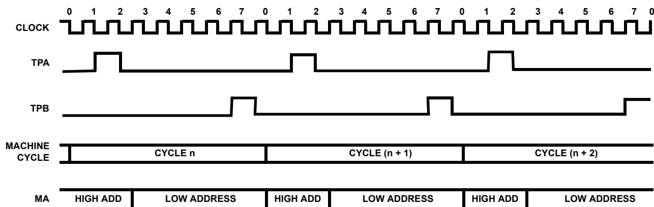
FIGURE 3. GENERAL TIMING WAVEFORMS
