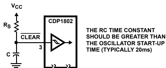
FIGURE 20. RESET DIAGRAM
