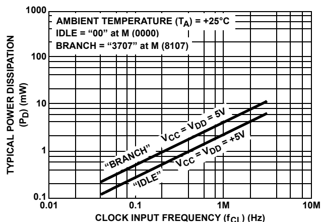
FIGURE 18. TYPICAL POWER DISSIPATION AS A FUNCTION OF CLOCK FREQUENCY FOR BRANCH INSTRUCTION AND IDLE INSTRUCTION
