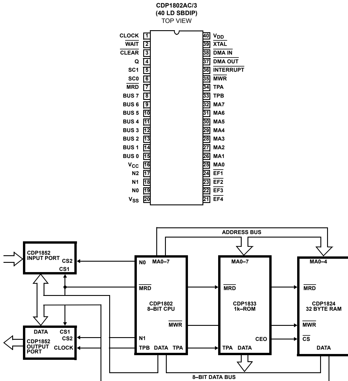
FIGURE 1. TYPICAL CDP1802A/3 SMALL MICROPROCESSOR SYSTEM
