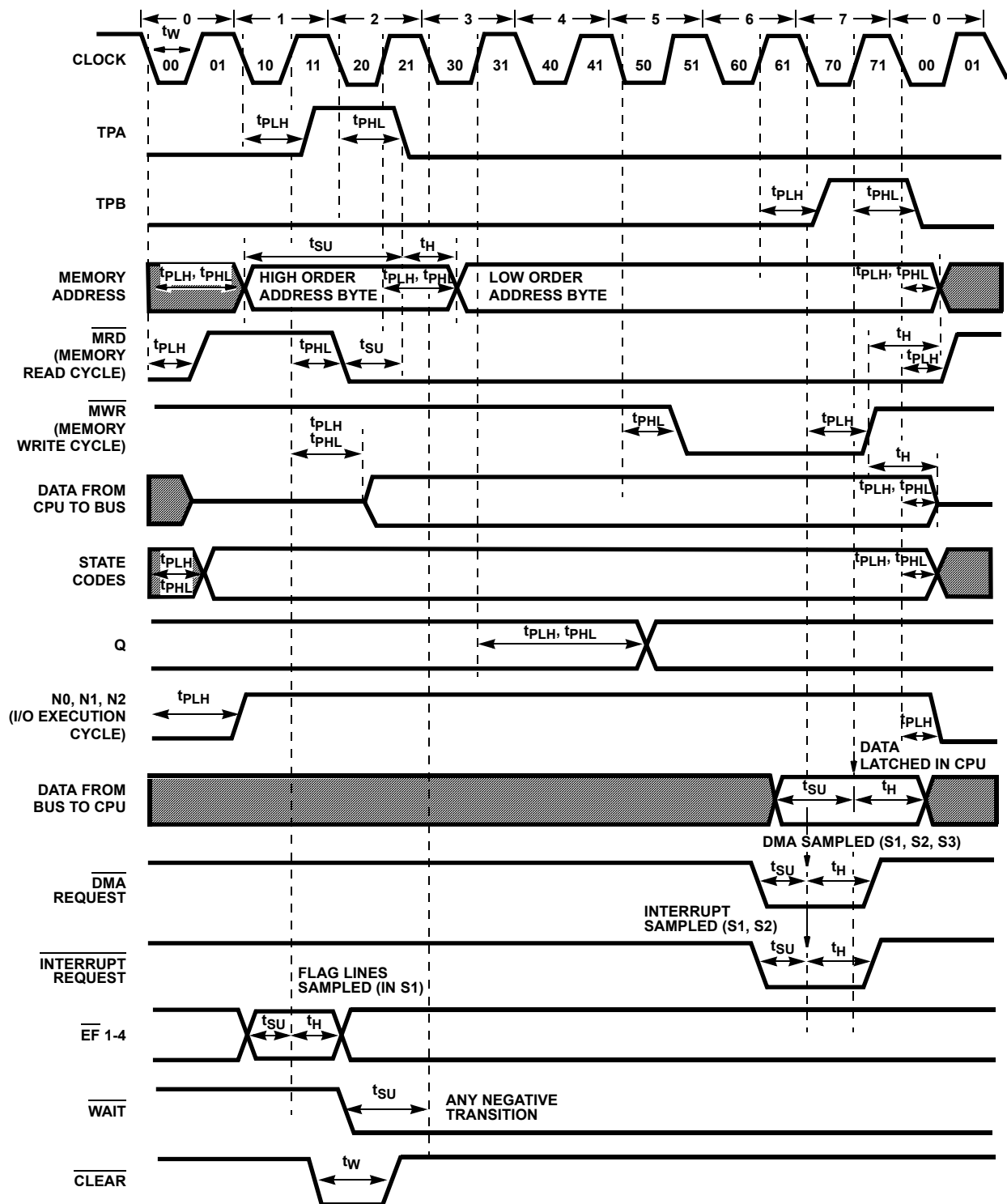
FIGURE 2. TIMING WAVEFORM
