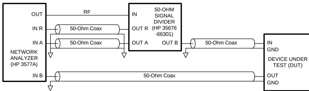
Test Setup
