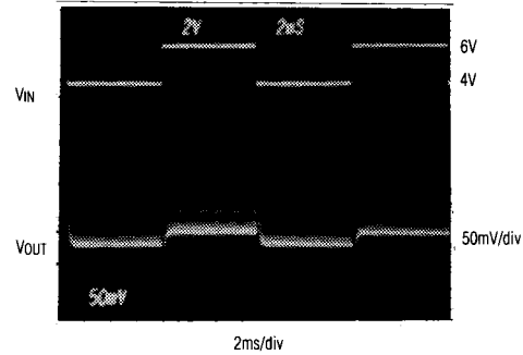
LINE-TRANSIENT RESPONSE
