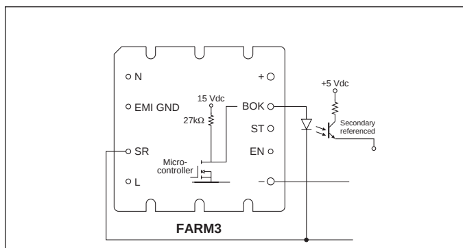
Figure 12—Bus OK (BOK) isolated power status indicator
