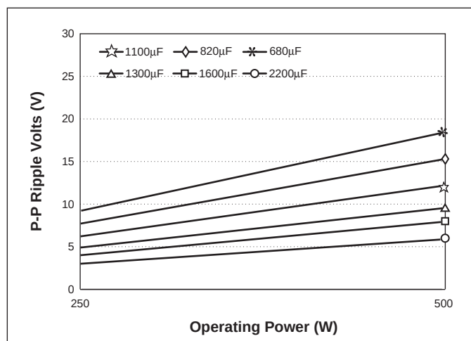
Figure 16—Ripple voltage vs. operating power and bus capacitance, series combination of C1, C2 (see Figure 1a)
