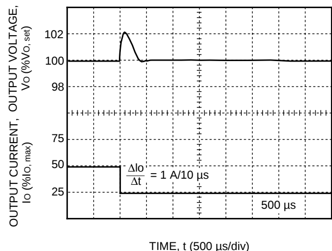
Figure 17. Typical A, B, C, D, F Output Voltage for a Step Load Change from 50% to 25%
