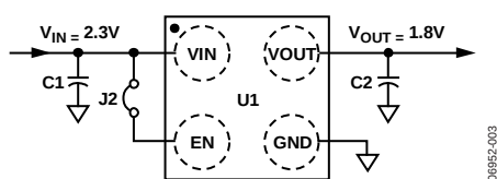
Figure 4. Evaluation Board Schematic, WLCSP
