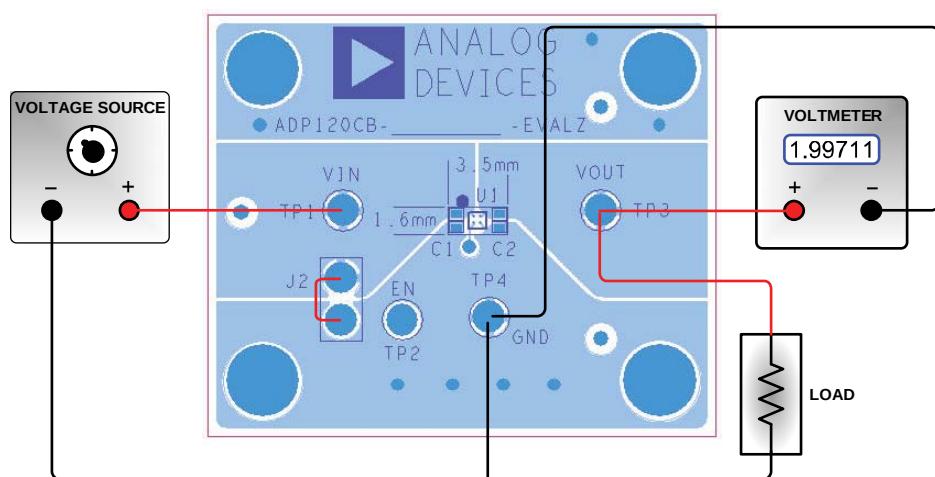
Figure 6. Output Voltage Measurement Setup, WLCSP
