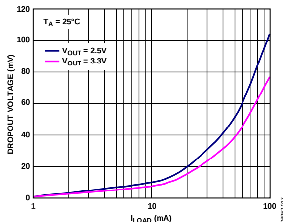
Figure 9. TSOT Dropout Voltages vs. Load Currents, I_{LOAD}
