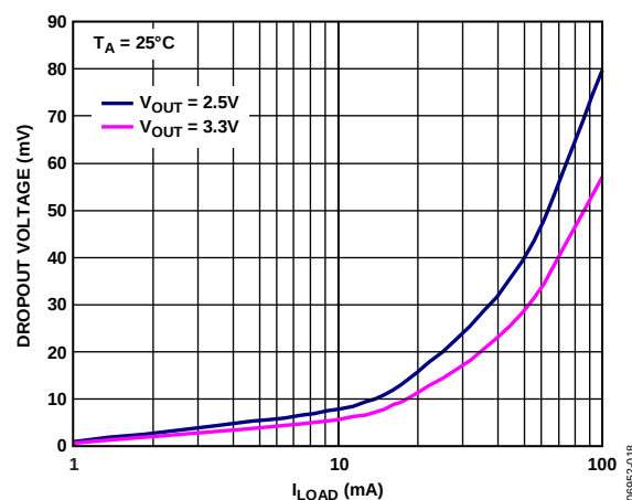
Figure 10. WLCSP Dropout Voltages vs. Load Currents, I_{LOAD}
