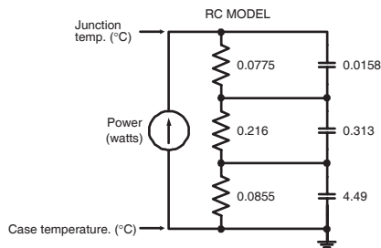
FIGURE 19b, TRANSIENT THERMAL IMPEDANCE MODEL
