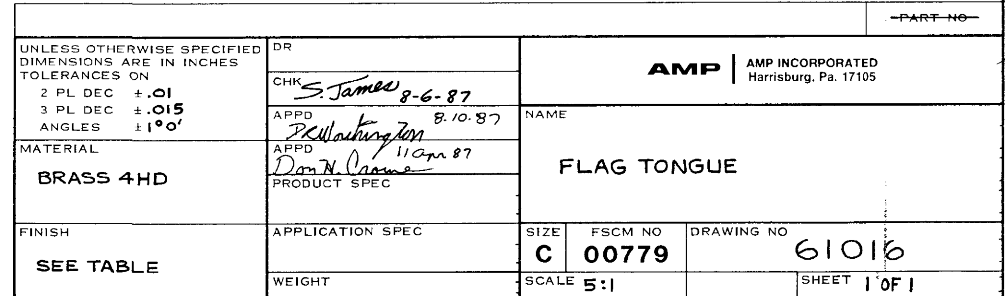
BRIGHT TIN 61016-3 MATTE TIN 61016-1 FINISH PART NUMBER
