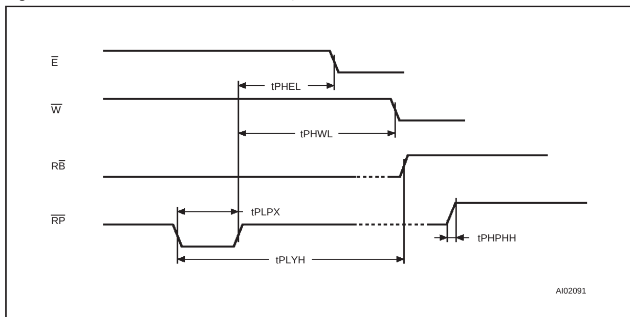
Figure 9. Read and Write AC Characteristics, \overline{R\overline{P}} Related
