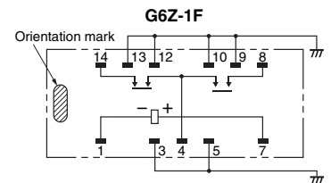
Terminal Arrangement/Internal Connections (Top View)
