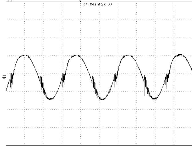
Figure 12: Output voltage ripple at nominal input voltage and rated load current ( I_o=5A ) (20mV/div, 1us/div) Load capacitance: 1 \mu F ceramic capacitor and 10 \mu F tantalum capacitor. Bandwidth: 20 MHz. Scope measurements should be made using a BNC cable (length shorter than 20 inches). Position the load between 51 mm to 76 mm (2 inches to 3 inches) from the module
