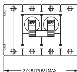
4-POLE (AB4)
