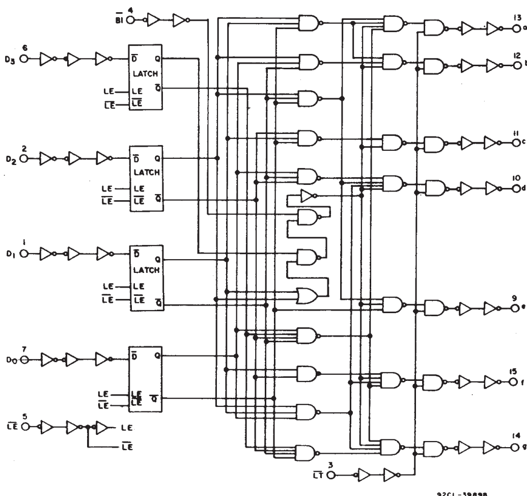
Fig. 1 - Logic diagram.
