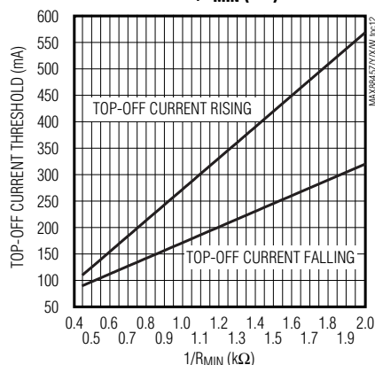
TOP-OFF CURRENT THRESHOLD vs. 1/R_{MIN} ( k\Omega )
