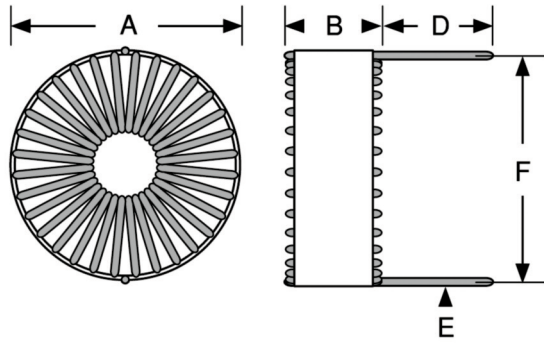
Horizontal Configuration
