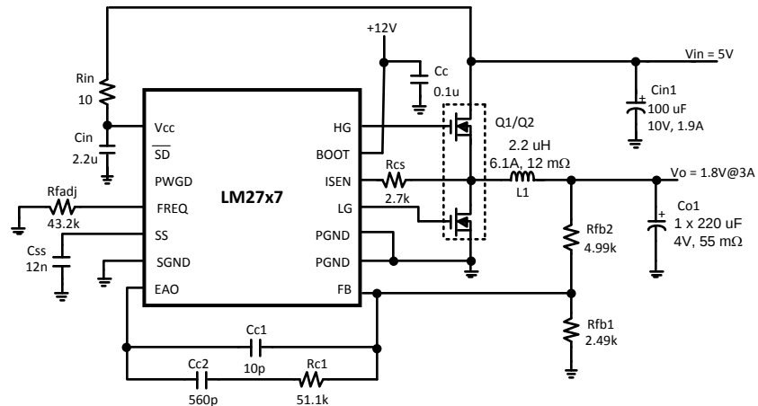
Figure 27. 5V to 1.8V, 3A, 600kHz
