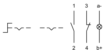
Wiring diagram 16
