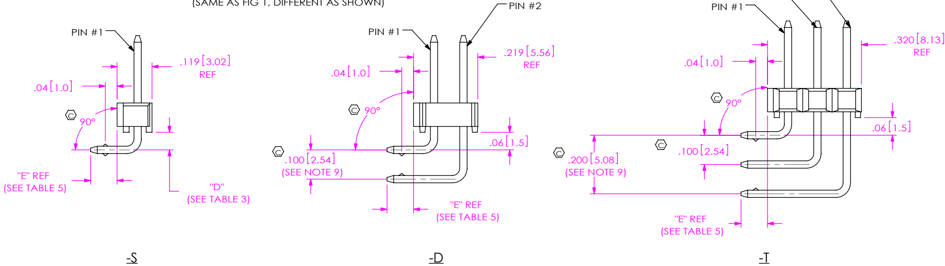
FIG 5 (RIGHT ANGLE) (-LA OPTION IS SHOWN ON ALL RIGHT ANGLES FOR DIMENSIONAL AND LOCATION PURPOSES.) (SEE CRIMP DETAIL VIEW, SHT 3) (SAME AS FIG 1, DIFFERENT AS SHOWN)
