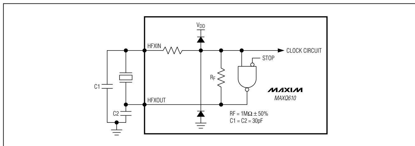
Figure 9. On-Chip Oscillator
