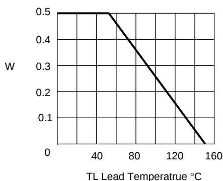
Figure 2 - Derating Curve
