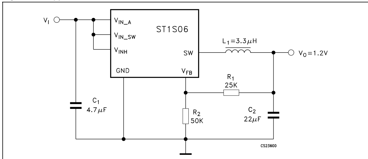
Figure 24. Application circuit
