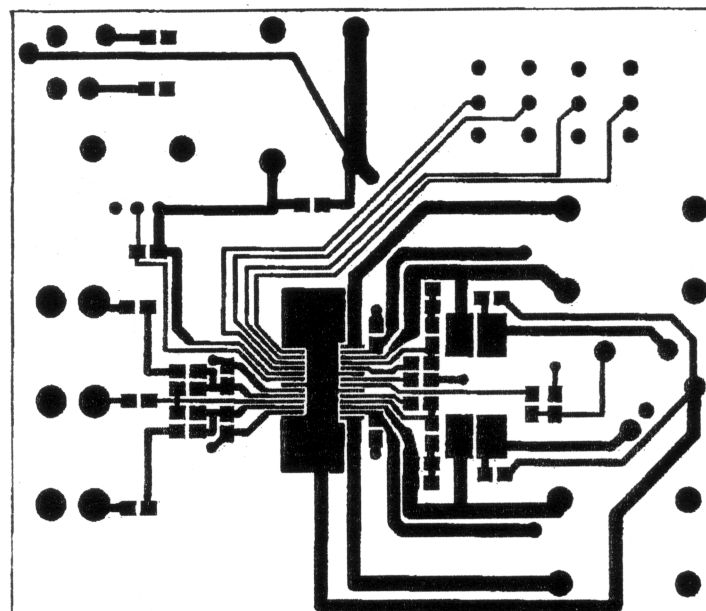
Figure 48. Top Layer TSSOP
