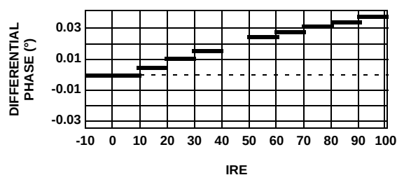
FIGURE 40. DIFFERENTIAL PHASE ERRORS
