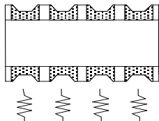
744C083 4 Resistors 8 Terminations
