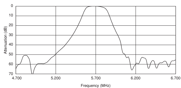
SFSKB5M70GF00-R1
