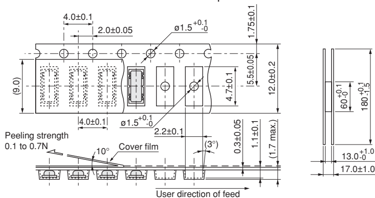
Dimensions of Carrier Tape
