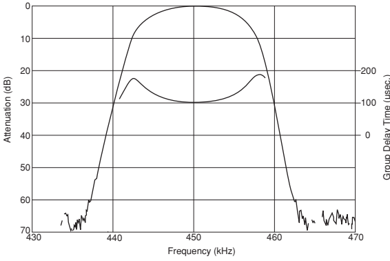
IFT+CFWLA450KF1Y-B0
