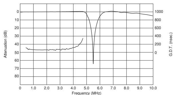
TPSKA5M50B00-R3
