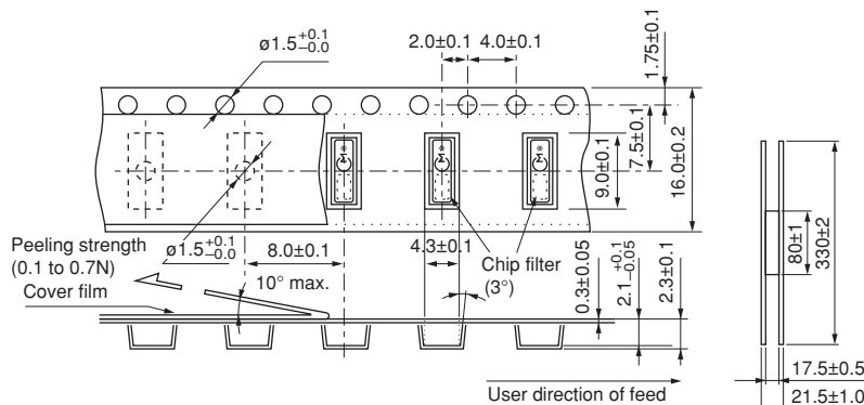
Dimensions of Carrier Tape
