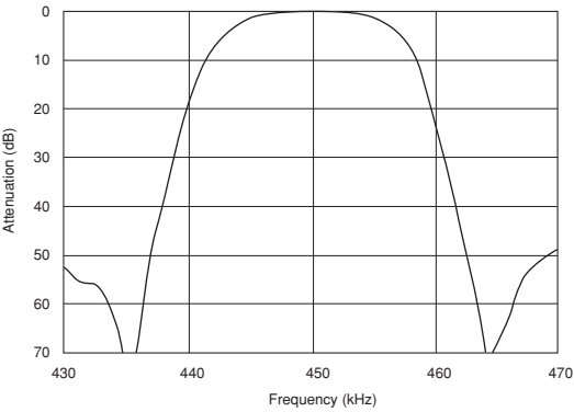
IFT+SFPLA450KF1A-B0
