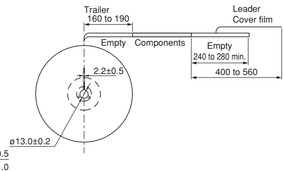
Dimensions of Reel
