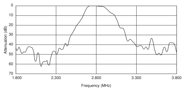
SFSKB2M80GF00-R1
