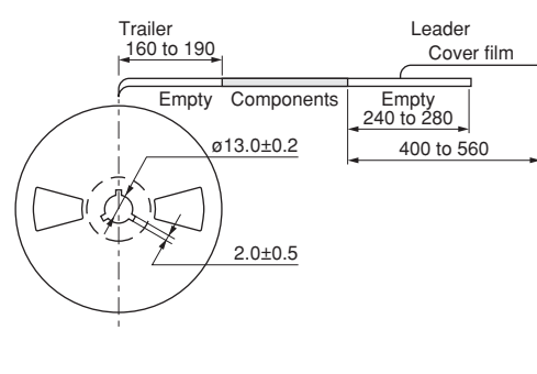
Dimensions of reel
