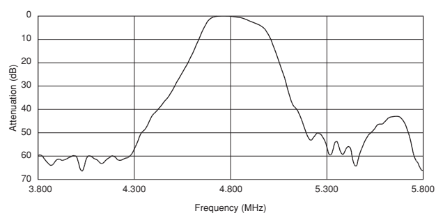
SFSKB4M80GF00-R1
