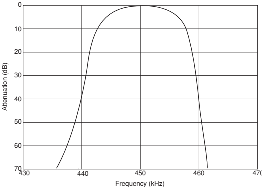
IFT+CFWLA450KFFA-B0
