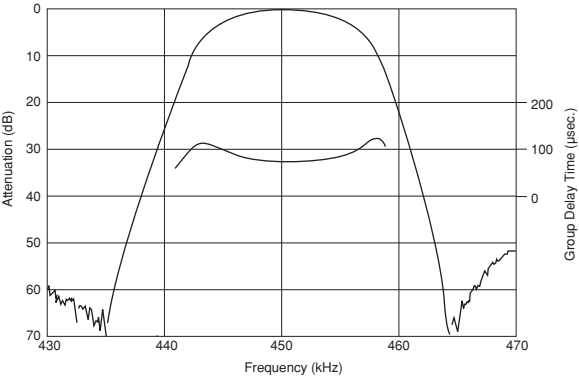
IFT+CFULA450KF1Y-B0
