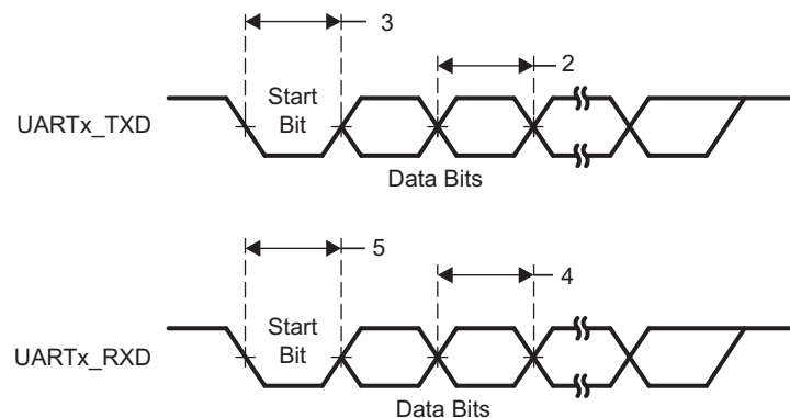
Figure 8-86. UART Timing
