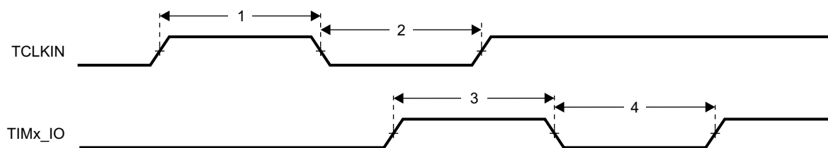
Figure 8-85. Timer Timing
