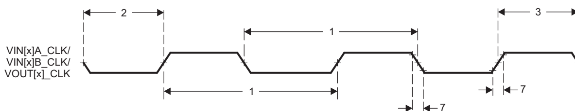
Figure 8-27. HDVPSS Clock Timing
