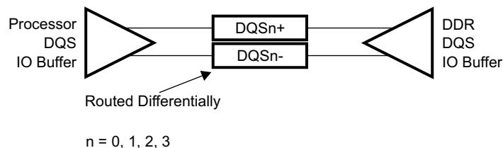
Figure 8-65. DQS Topology
