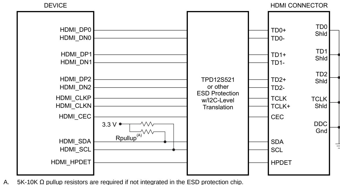
Figure 8-26. HDMI Interface High-Level Schematic
