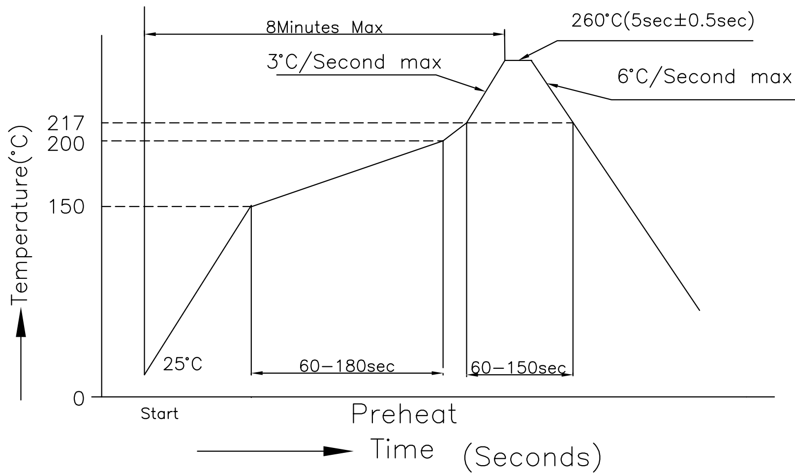
LCP Recommended Temperature Profile
