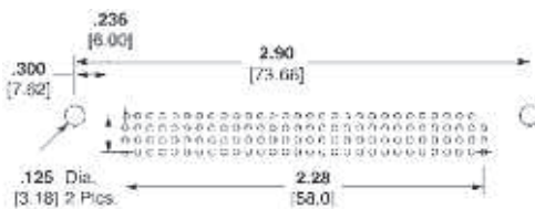
Recommended PC Board Layout for 1375797-3, 1375797-6, 1375798-3, 1375798-6
