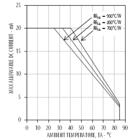
Figure 7 Derating Curve
