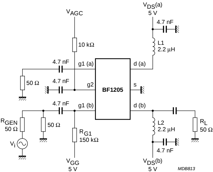
Fig.30 Cross-modulation test set-up for amplifier b.
