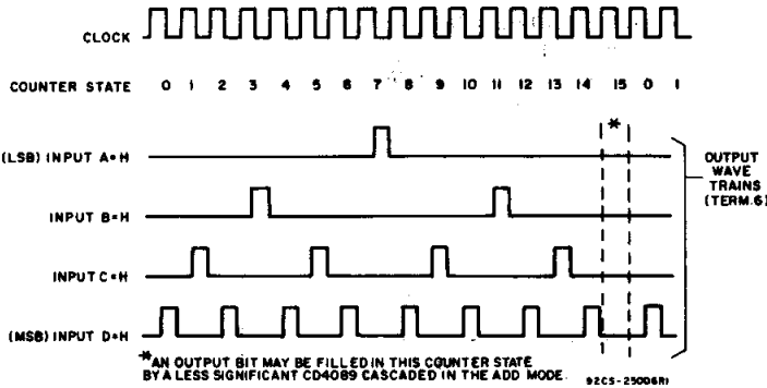
Fig. 15 - Timing diagram.
