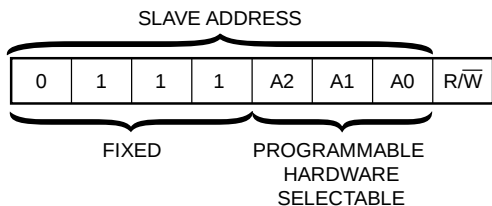
Figure 7. CAT9554A Slave Address
