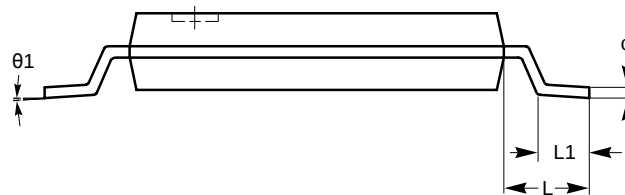
END VIEW
