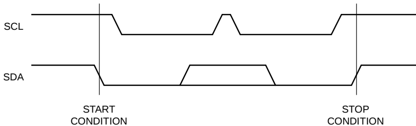
Figure 5. START/STOP Condition
