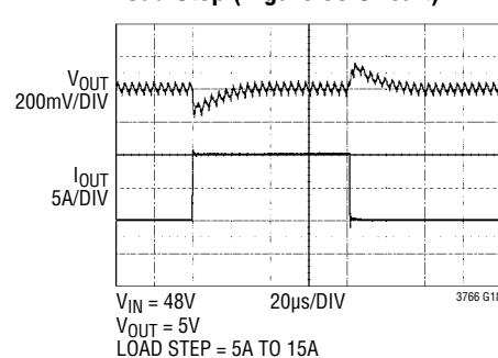
Load Step (Figure 39 Circuit)
